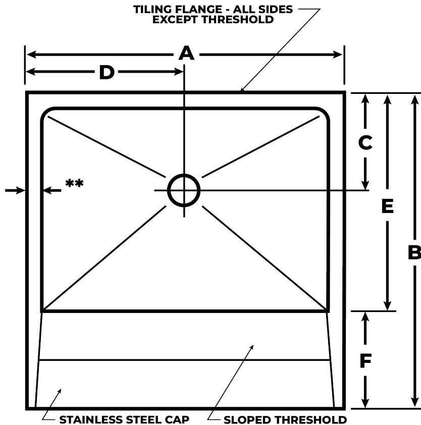
PLAN "WS" SERIES W/ 3" CURB**
