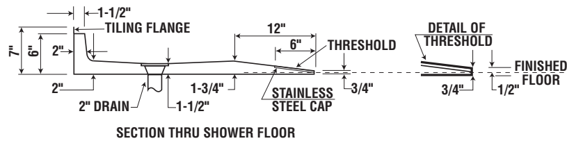
SECTION THRU SHOWER FLOOR
