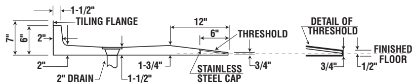
SECTION THRU SHOWER FLOOR
