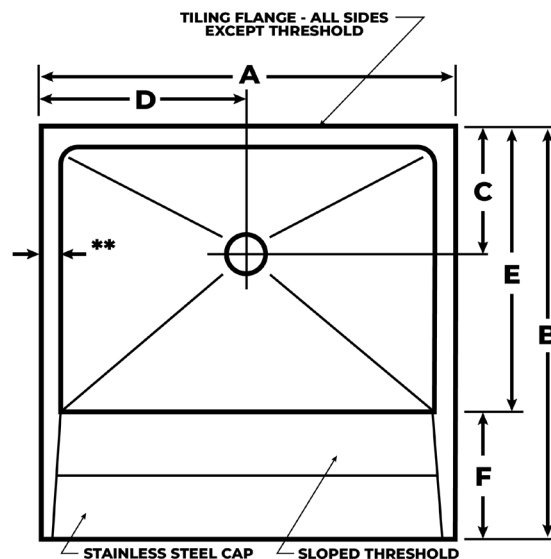
PLAN "WS" SERIES W/ 3" CURB**
